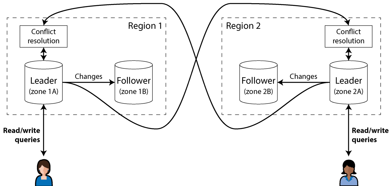
Figure 6-6. Multi-leader replication across multiple regions
