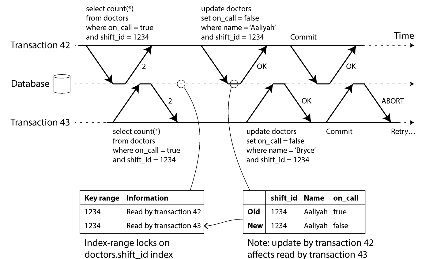
Figure 8-11. In serializable snapshot isolation, detecting when one transaction modifies another transaction’s reads
