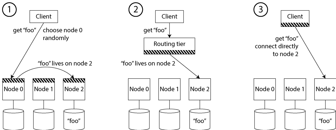
Figure 7-7. Three ways of routing a request to the right node
