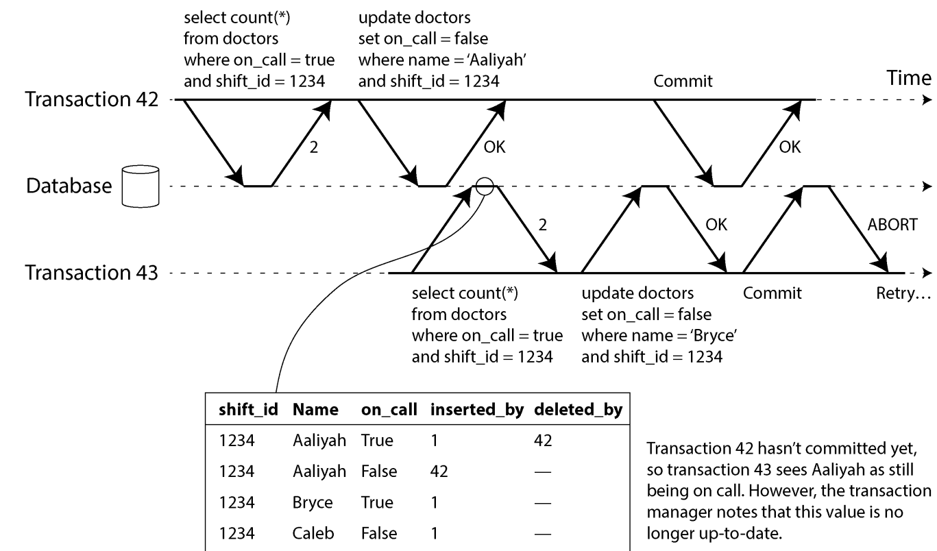
Figure 8-10. Detecting when a transaction reads outdated values from an MVCC snapshot
