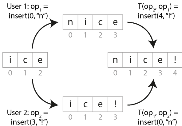
Figure 6-11. How two concurrent insertions into a string are merged by OT and a CRDT, respectively
