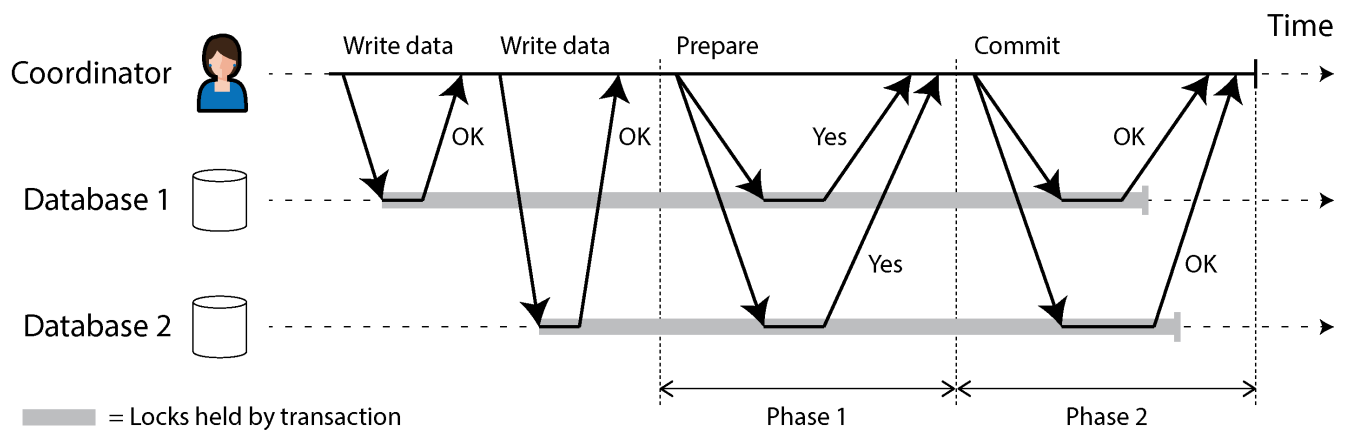
Figure 8-13. A successful execution of 2PC
