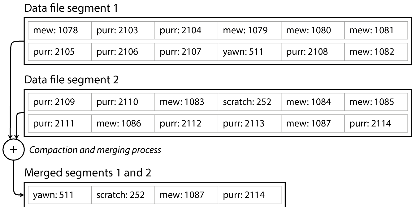
Figure 12-6. In this log of key-value pairs, the key is the ID of a cat video ( mew , purr , scratch , or yawn ) and the value is the number of times it has been played; log compaction retains only the most recent value for each key.
