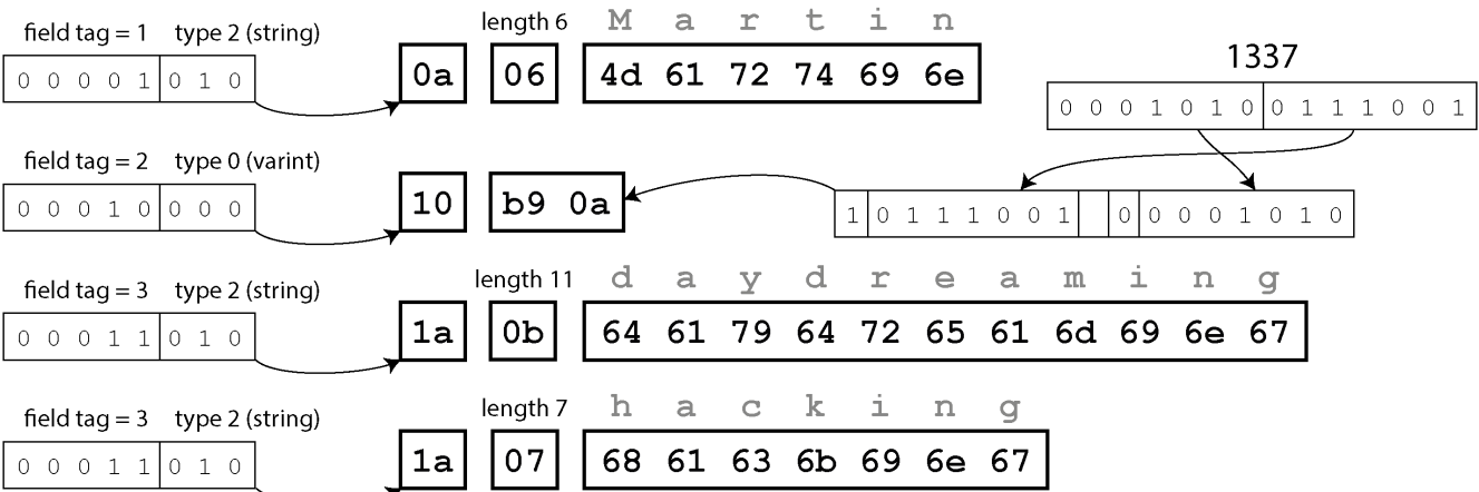
Figure 5-3. Our record encoded using Protocol Buffers
