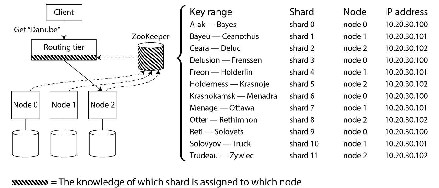
Figure 7-8. Using ZooKeeper to keep track of the assignment of shards to nodes
