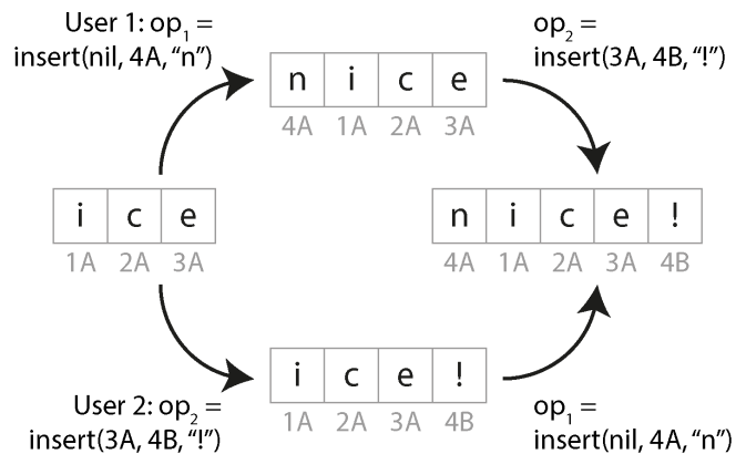
Figure 6-11. How two concurrent insertions into a string are merged by OT and a CRDT, respectively
