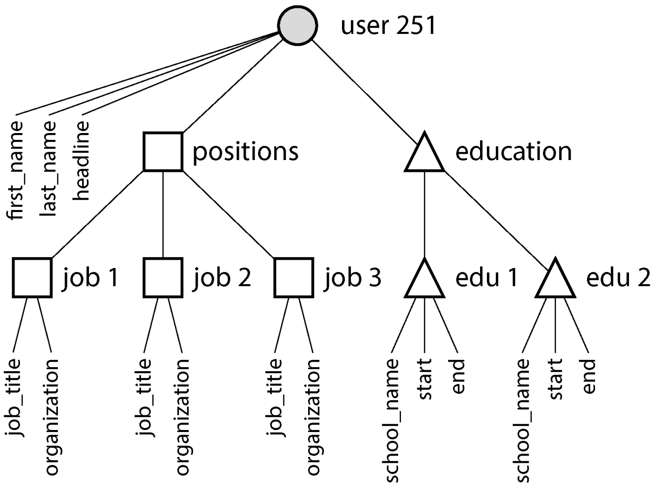
Figure 3-2. One-to-many relationships forming a tree structure
