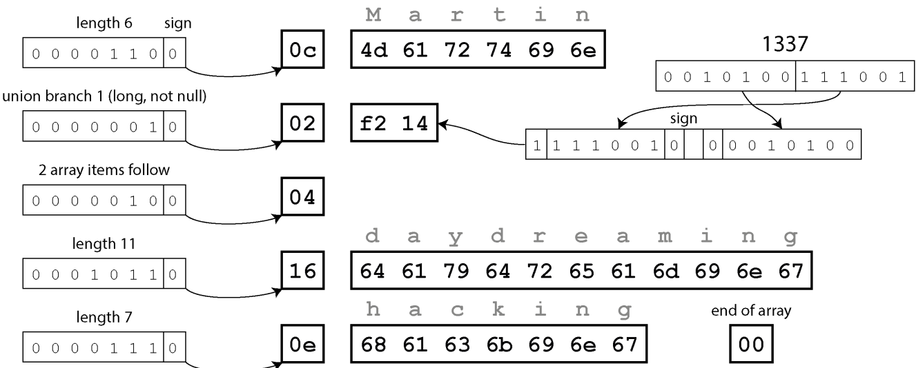
Figure 5-4. Our record encoded using Avro
