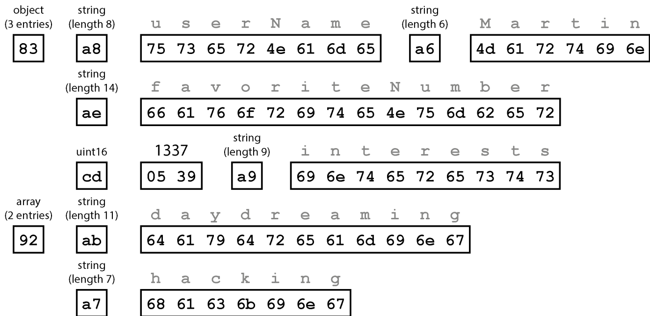
Figure 5-2. Our record ( Example 5-2 ) encoded using MessagePack
