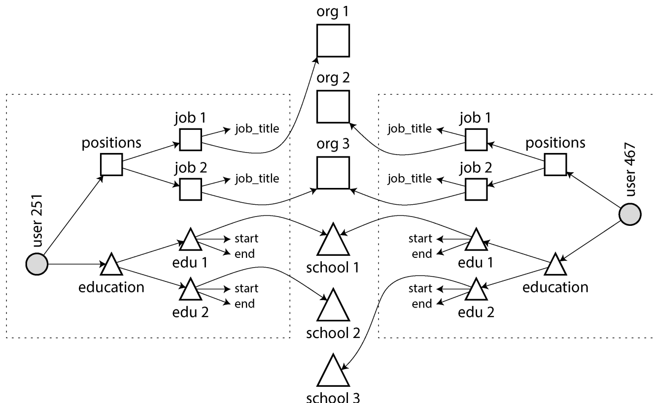
Figure 3-4. Many-to-many relationships in the document model—the data within each dotted box can be grouped into one document
