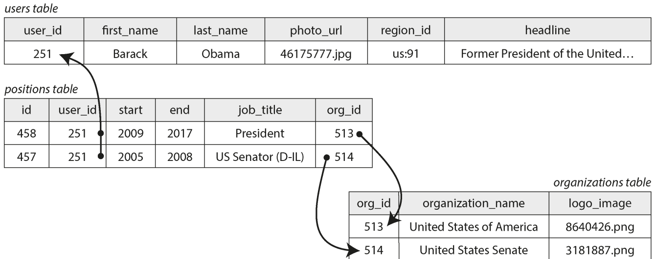
Figure 3-3. Many-to-many relationships in the relational model
